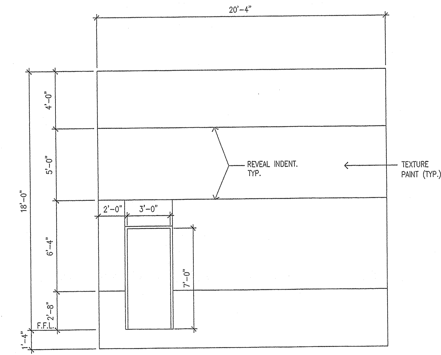
6 PANEL TYPE "N-2" A-12 1/4" = 1'-0"
