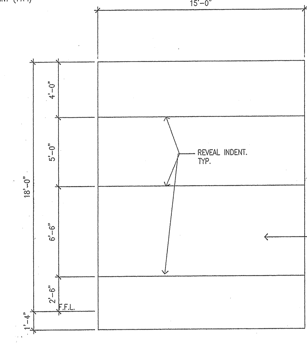
4 PANEL TYPE "M" A-12 1/4" = 1'-0"
