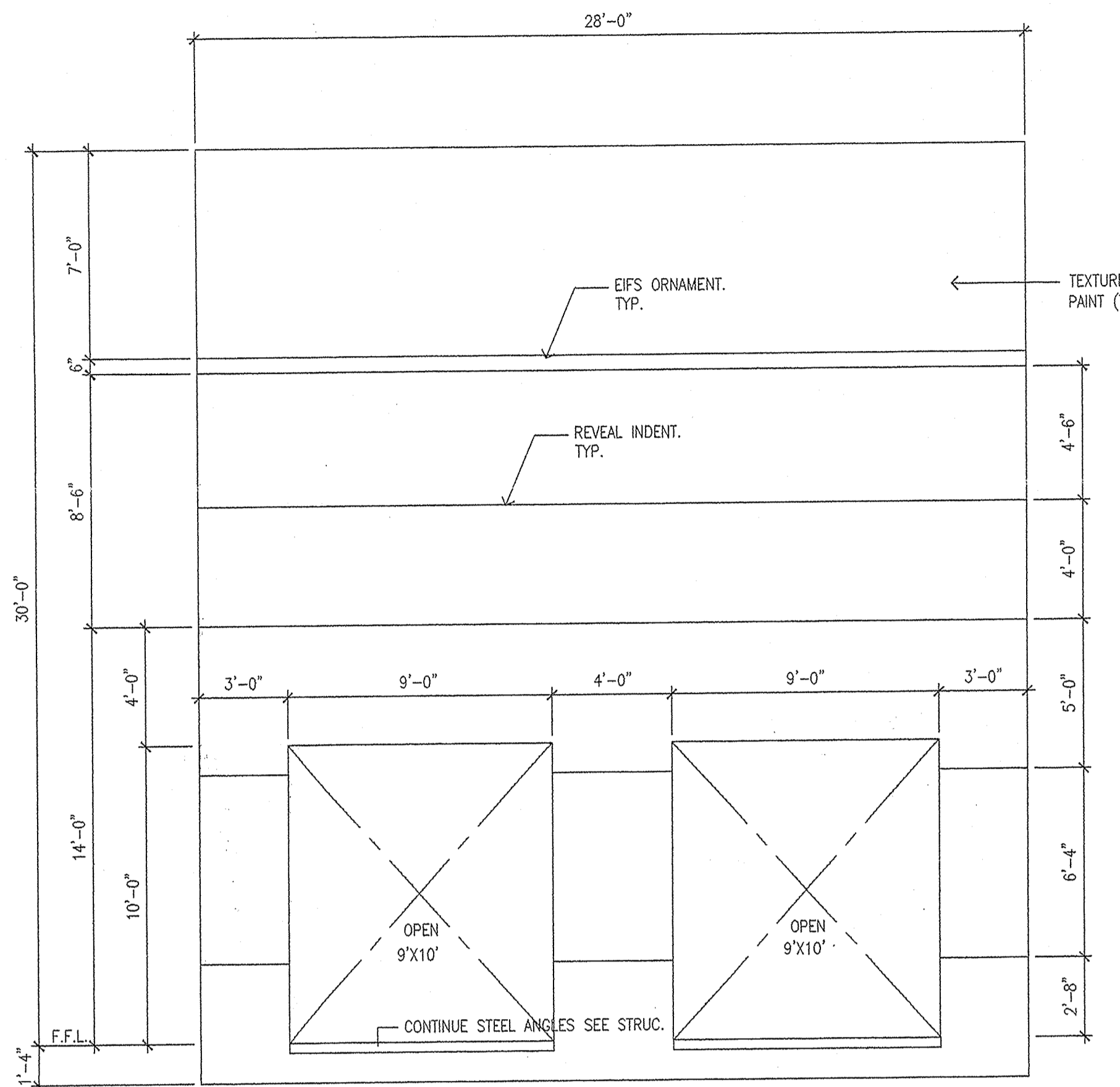
1 PANEL TYPE "J" A-12 1/4" = 1'-0"
