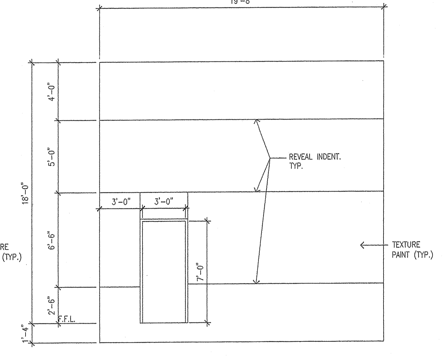
5 PANEL TYPE "N-1" A-12 1/4" = 1'-0"
