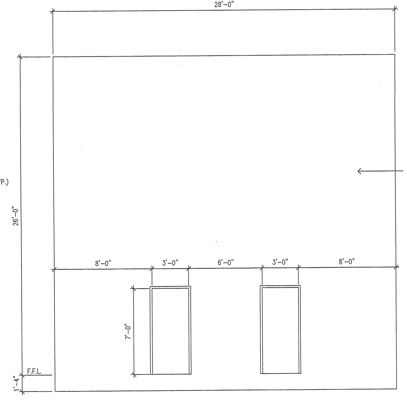
9 PANEL TYPE "R" A-12 1/4" = 1'-0"
