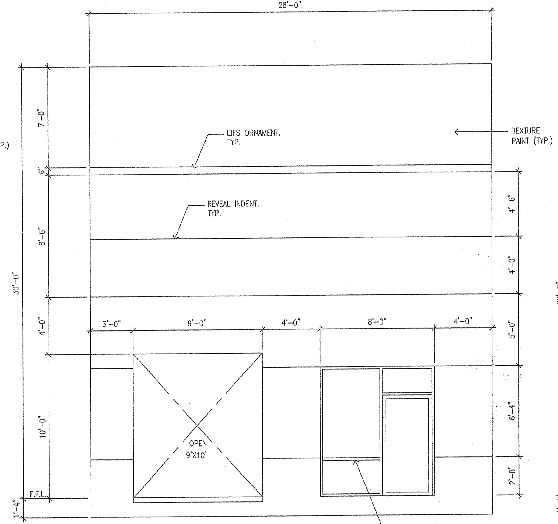
2 PANEL TYPE "K" A-12 1/4" = 1'-0"
