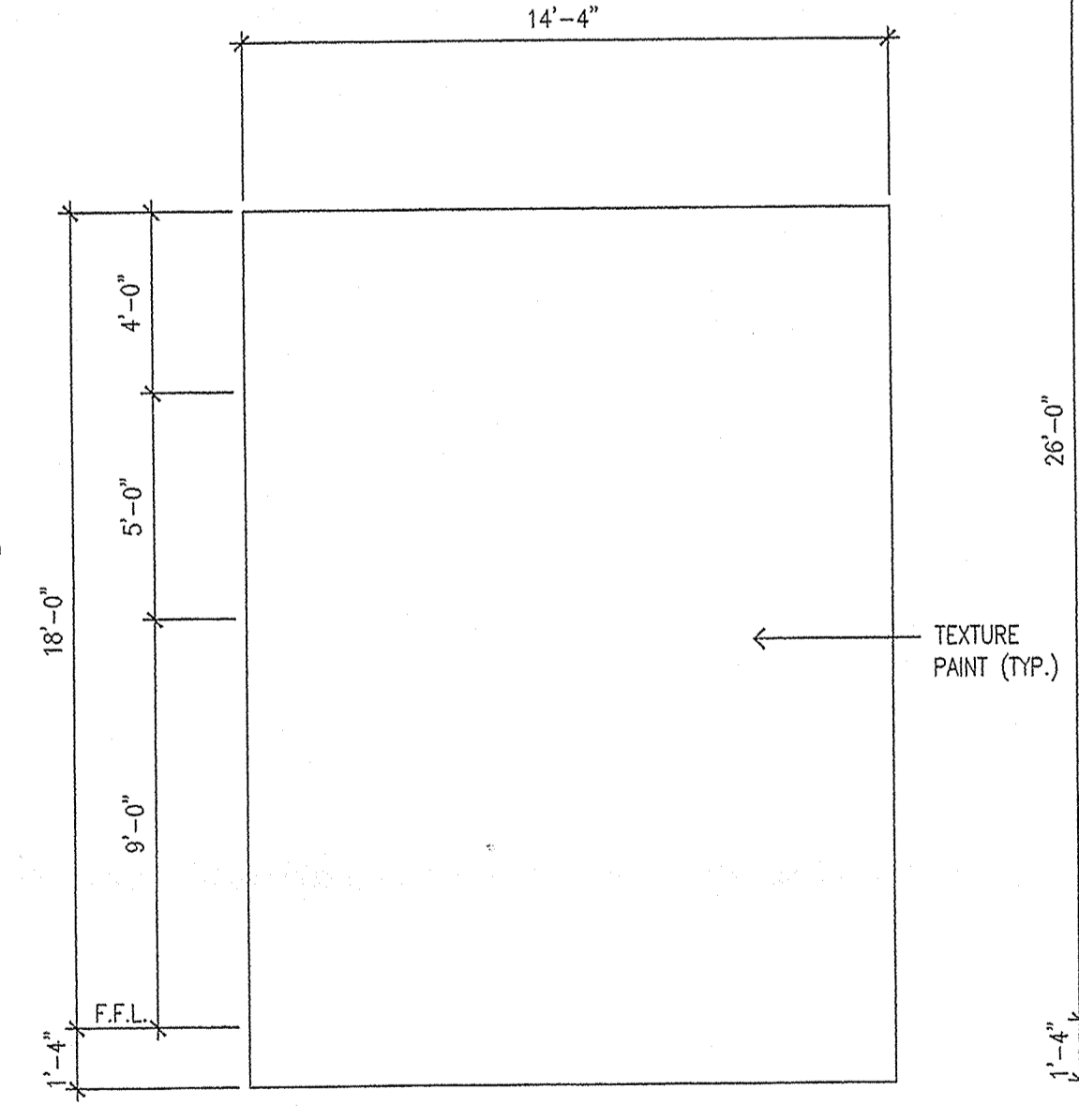
7 PANEL TYPE "P" A-12 1/4" = 1'-0"
