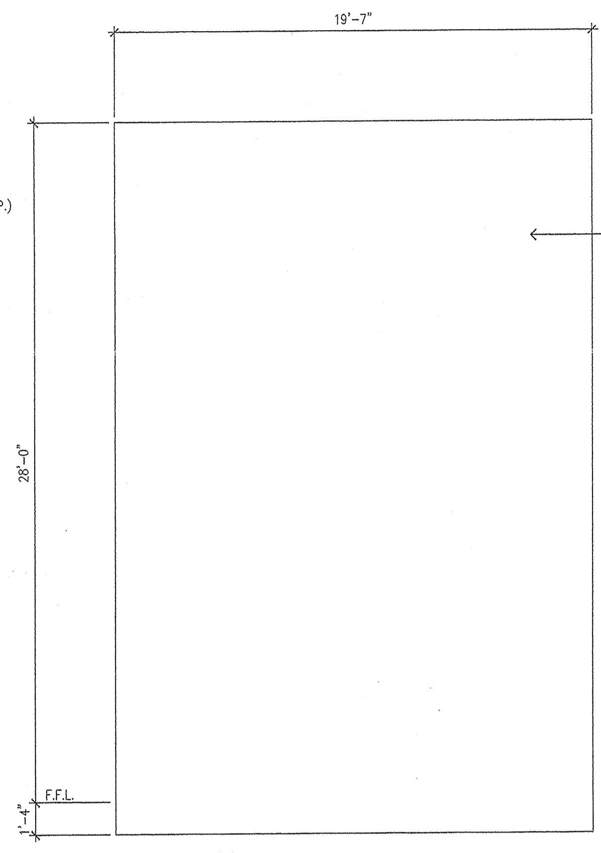
3 PANEL TYPE "L" A-12 1/4" = 1'-0"
