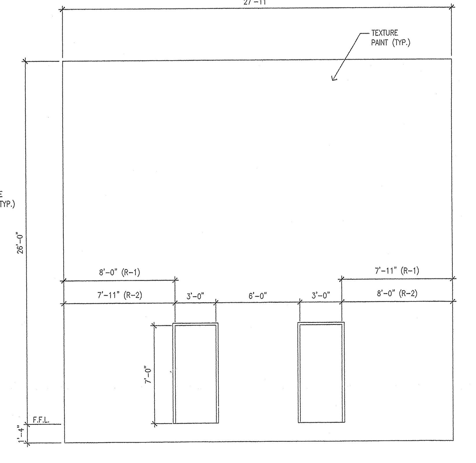
10 PANEL TYPE "R-1" & "R-2" A-12 1/4" = 1'-0"
