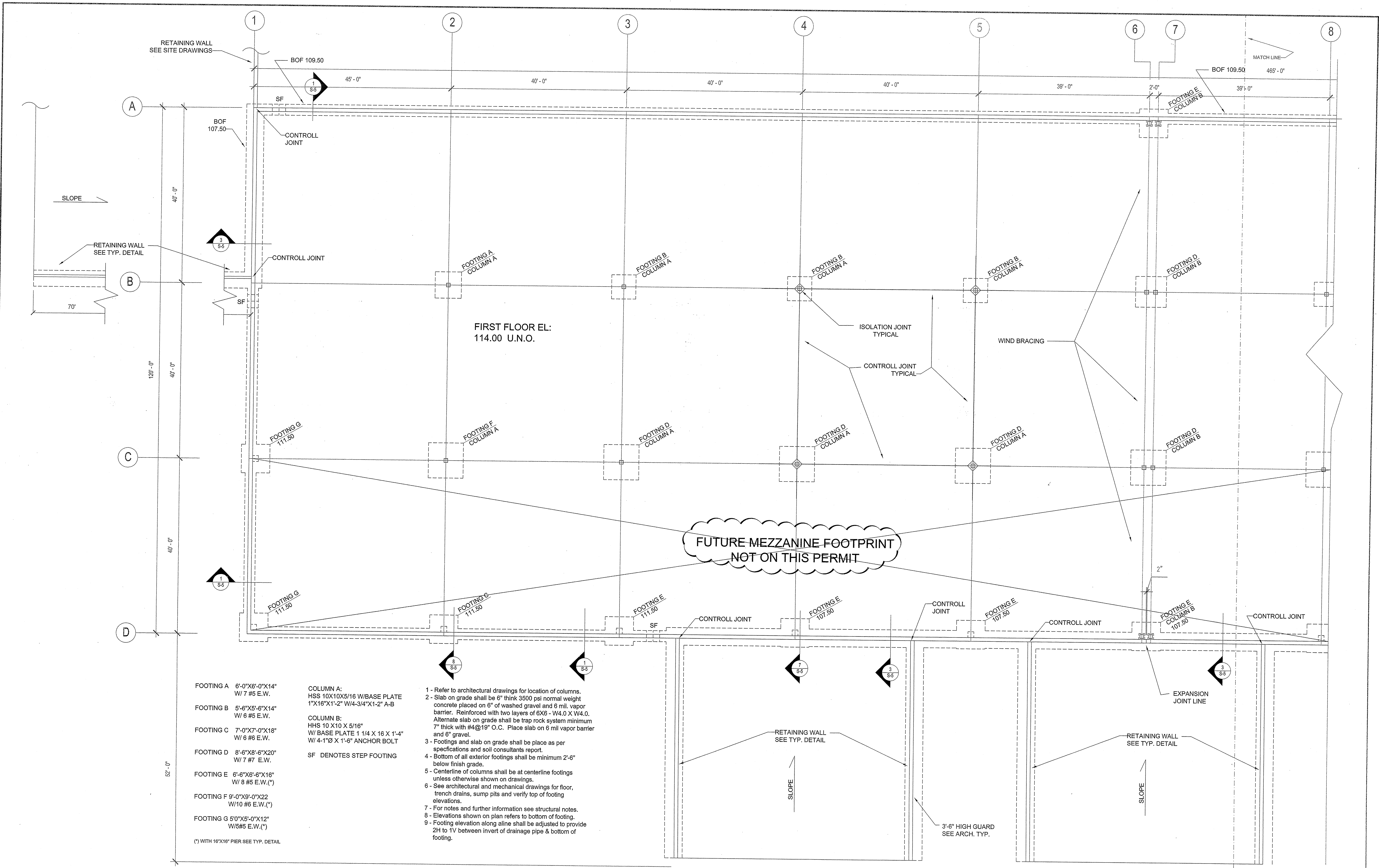
PARTIAL FOUNDATION PLAN SCALE: 1/8" = 1'-0"
